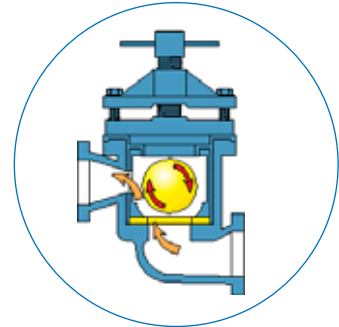
Biased flow in the ball valve housing balances out the wear on the ball thereby prolonging valve life.
